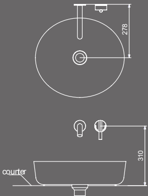
Wall - mount two hole faucet mixer and above counter basin
